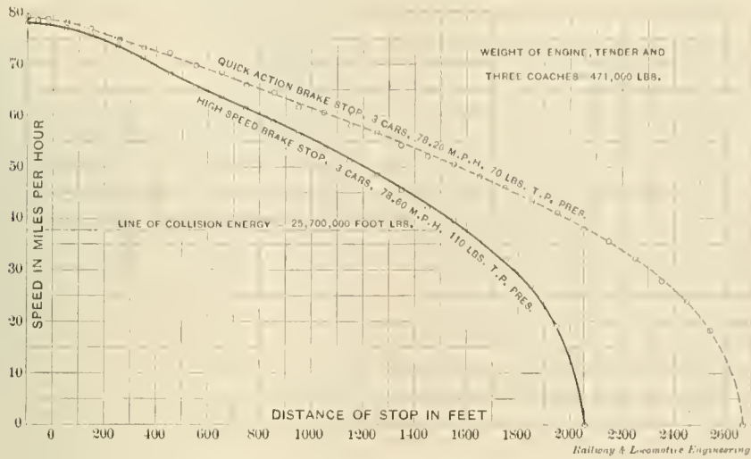
FIG. 4.—CARD SHOWING VALUE OF HIGH-SPEED BRAKE OVER ORDINARY BRAKE. Better stop made by High-Speed Brake, 610 feet. Collision speed, 36 miles per hour. Collision energy, 25,700,000 foot pounds.
